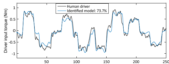
Example of driver torque T_d fitting under shared control.
