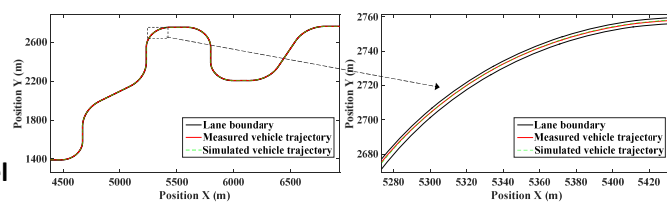
Example of comparison in vehicle trajectory
